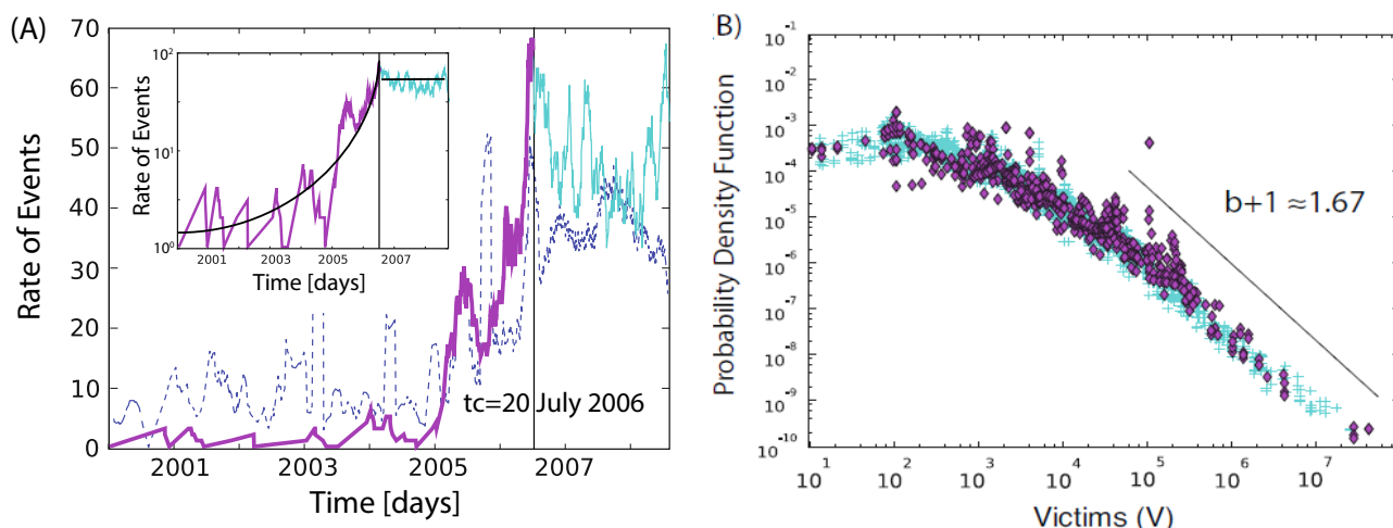
Figure 3: Frequency and severity distribution (Maillart and Sornette, 2010)
